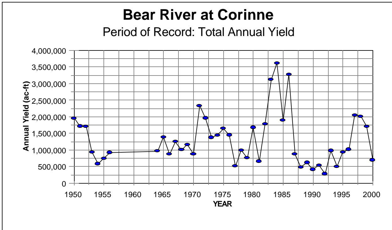
Figure 2-15. The annual water yield from the Bear River at Corinne from 1950 to 2000.
