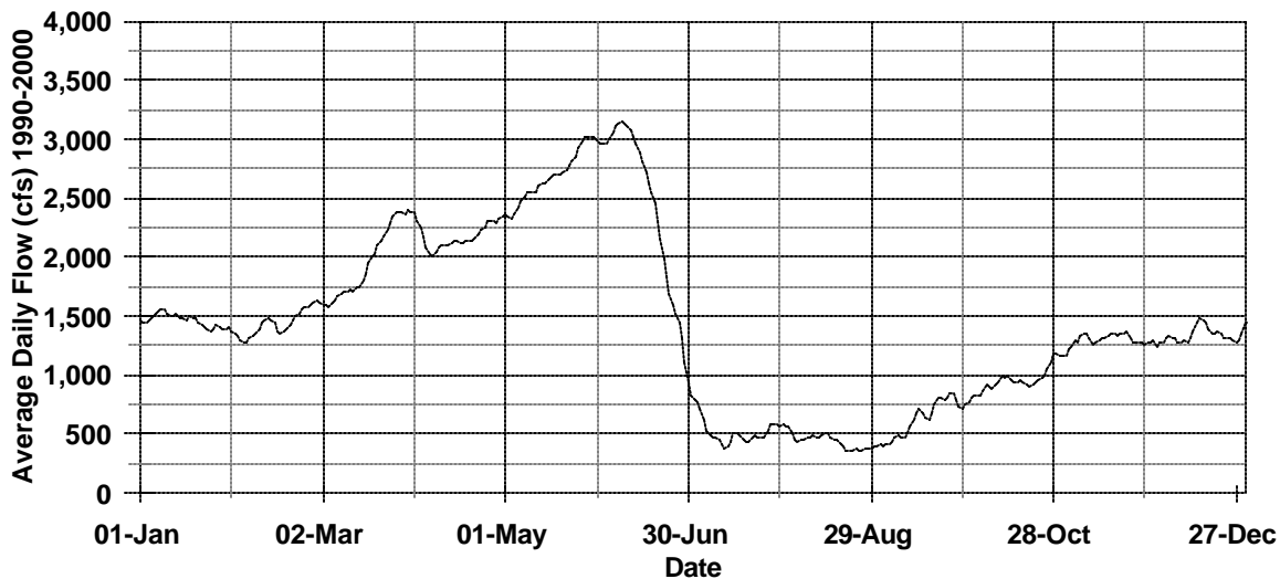
Figure 4-1. The flows in the Bear River at Corinne (Station No. 10126000) for the period of record (above) and the daily average for the 10 year period (below).
