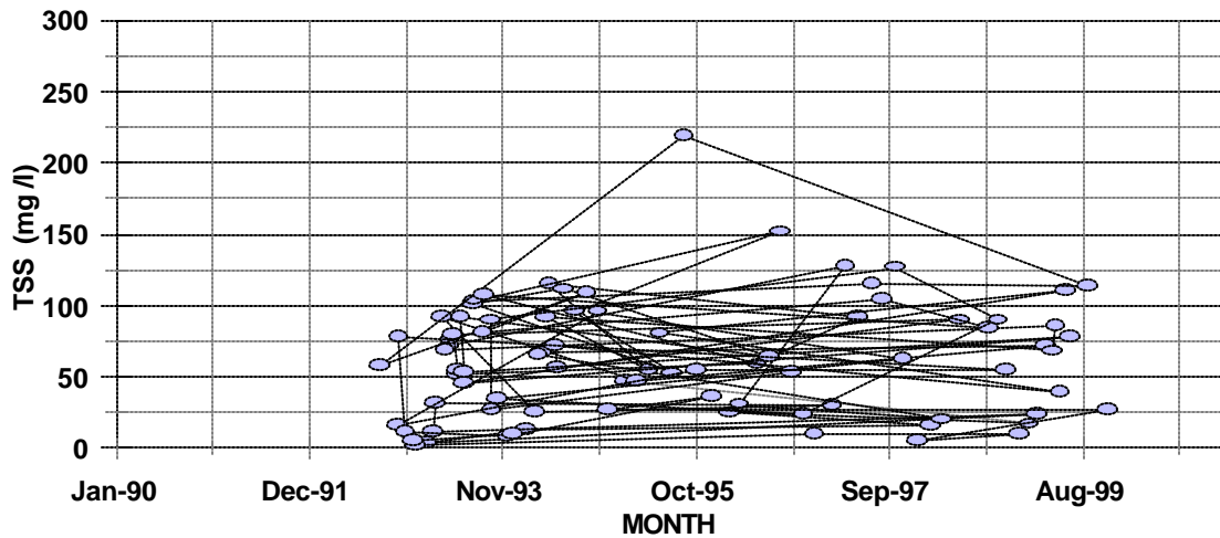
Figure 3-4. The concentration of total phosphorous (above) and total suspended solids (below) in the Bear River at Honeyville (Storet# 490170).
