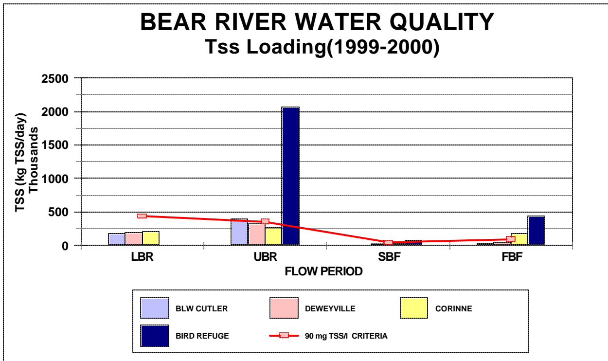
Figure 4-19. The daily loading in the Bear River for total phosphorus (above) and total suspended solids (below) during four hydrologic time periods (LBR=lower basin runoff; UBR=upper basin runoff; SBF=summer baseflow; and FBF=fall baseflow). Criteria are indicator values and not a standard.
