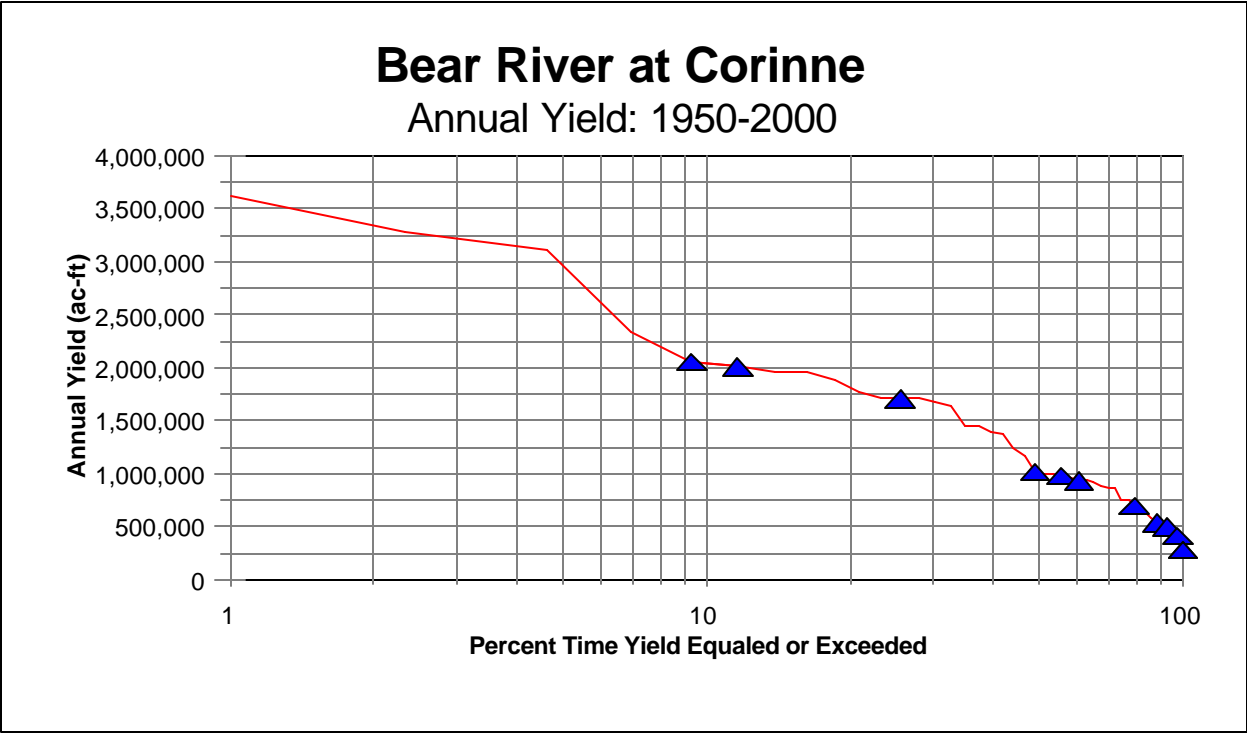
Figure 4-2. The annual flow yield exceedence curve with the ten years (1990-2000) of water quality data plotted as a comparison.
